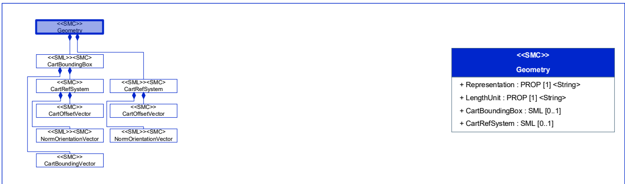
Figure 83: [Prop] LengthUnit
