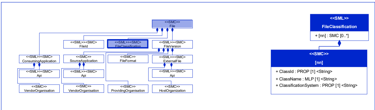
Figure 66: [MLP] ClassName
