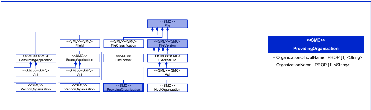
Figure 51: [Prop] OrganizationName
