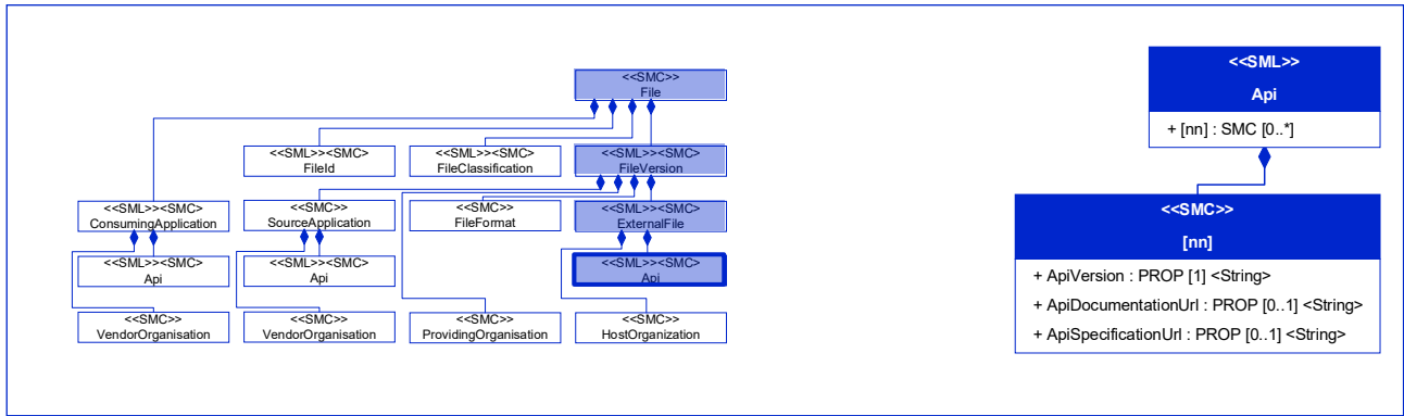
Figure 34: [Prop] ApiSpecificationUrl
