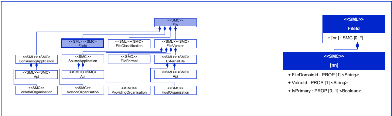
Figure 14: [Prop] IsPrimary
