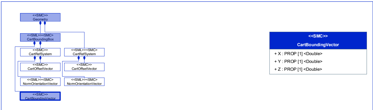
Figure 98: [Prop] Z
