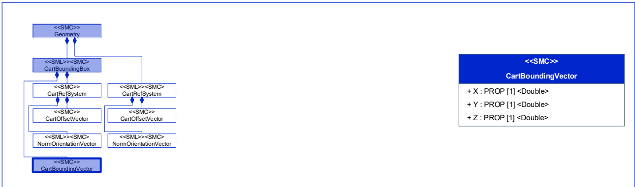
Figure 96: [Prop] X
