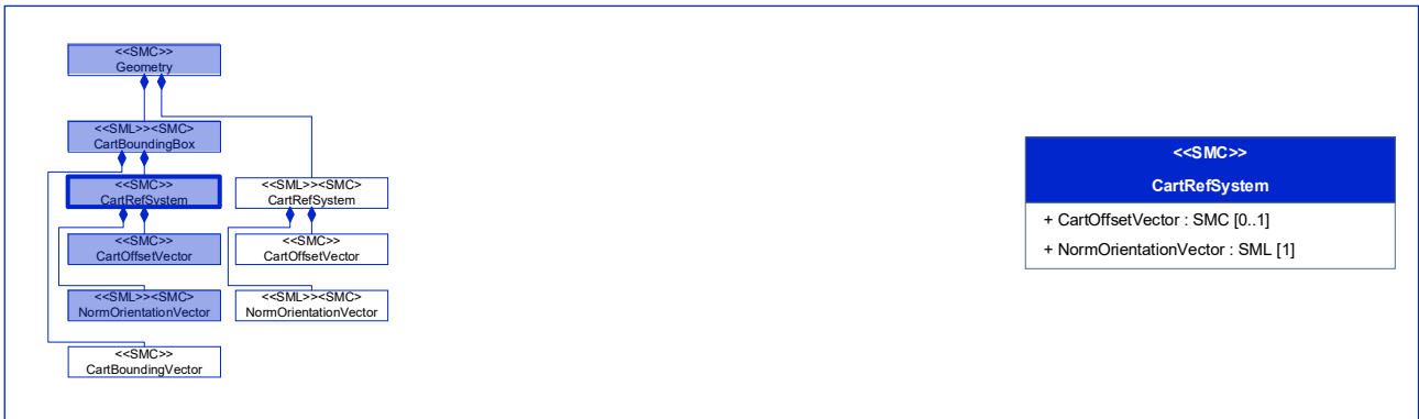
Figure 86: [SMC] CartRefSystem
