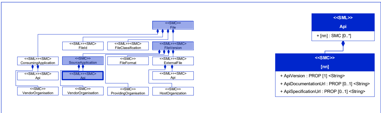
Figure 45: [Prop] ApiDocumentationUrl
