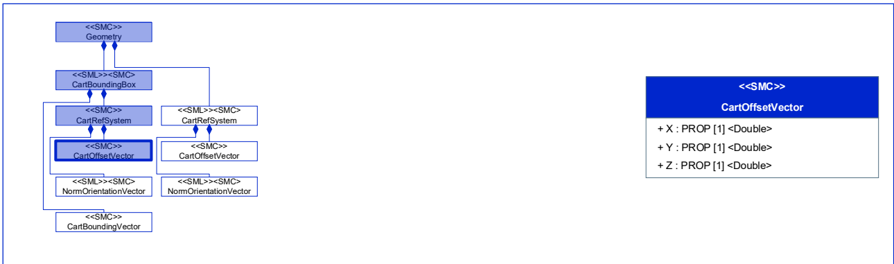
Figure 88: [Prop] X
