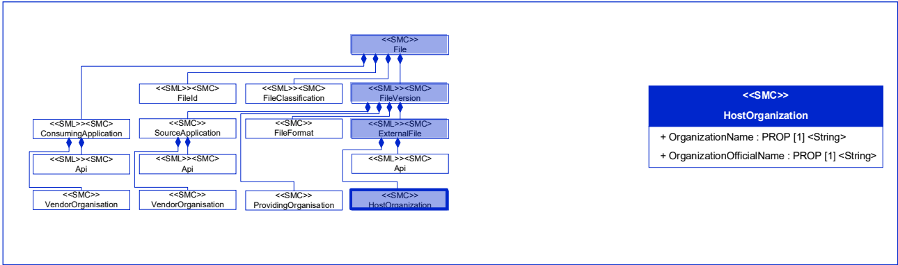
Figure 28: [SMC] HostOrganization
