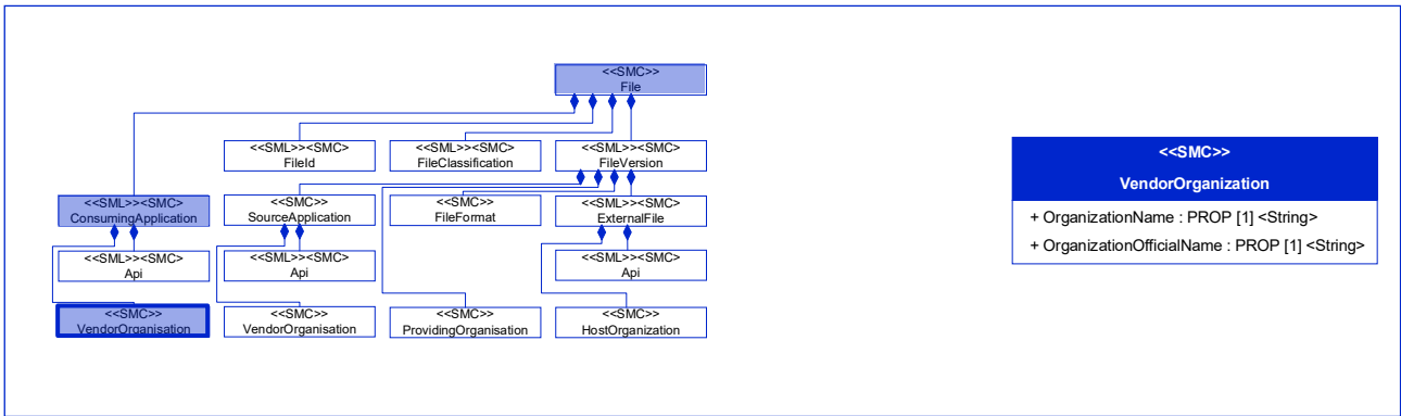
Figure 62: [Prop] OrganizationName
