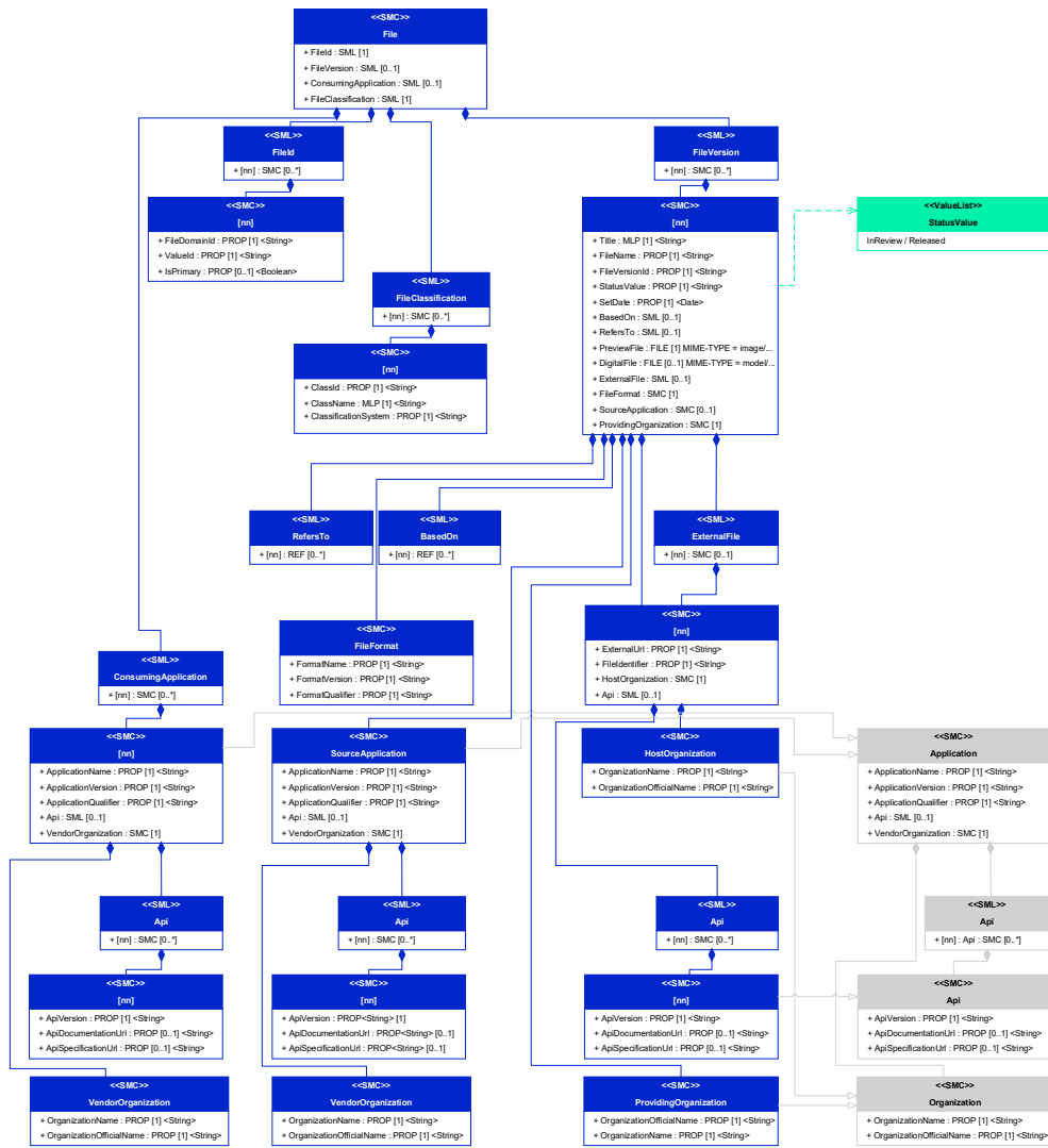
Figure 9: [SMC] File
