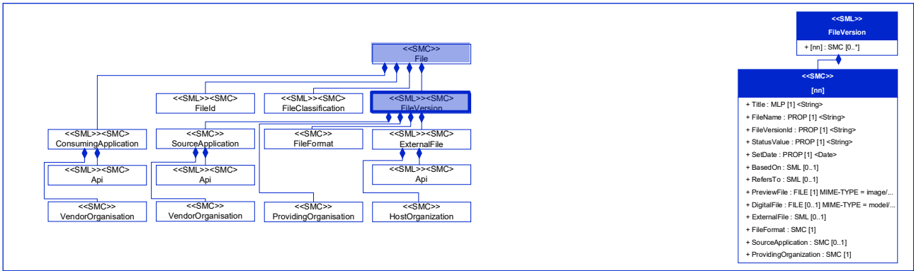
Figure 21: [SML][Ref] BasedOn
