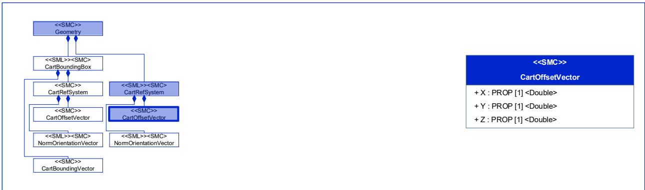
Figure 102: [Prop] Y
