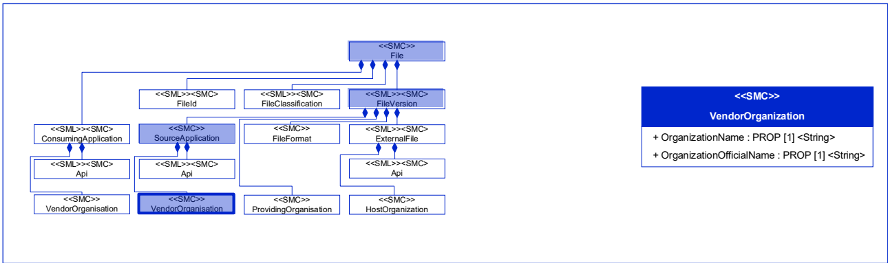
Figure 47: [SMC] VendorOrganization
