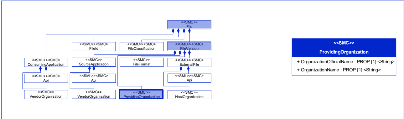
Figure 50: [SMC] ProvidingOrganization
