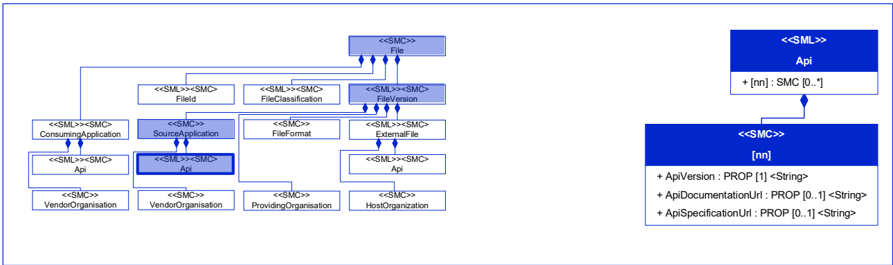
Figure 44: [Prop] ApiVersion
