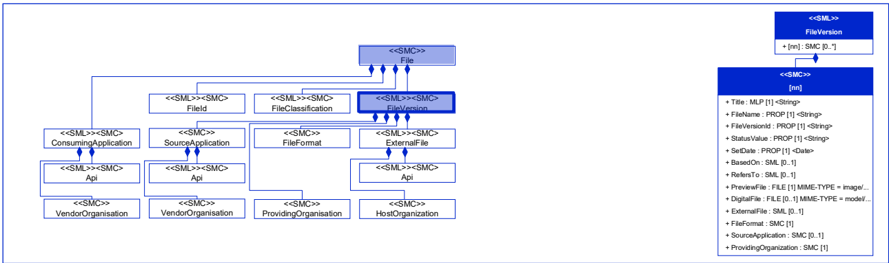
Figure 17: [Prop] FileName
