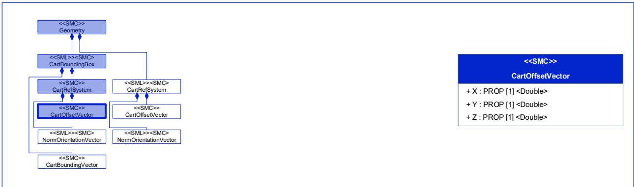
Figure 90: [Prop] Z
