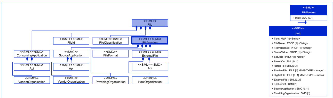
Figure 18: [Prop] FileVersionId
