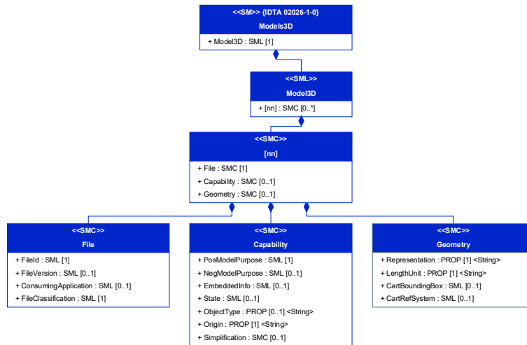
Figure 6: [SM] Models3D
