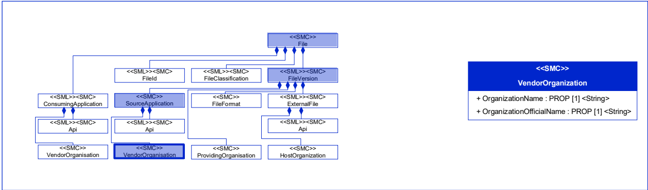
Figure 49: [Prop] OrganizationOfficialName
