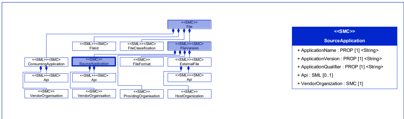
Figure 42: [Prop] ApplicationQualifier
