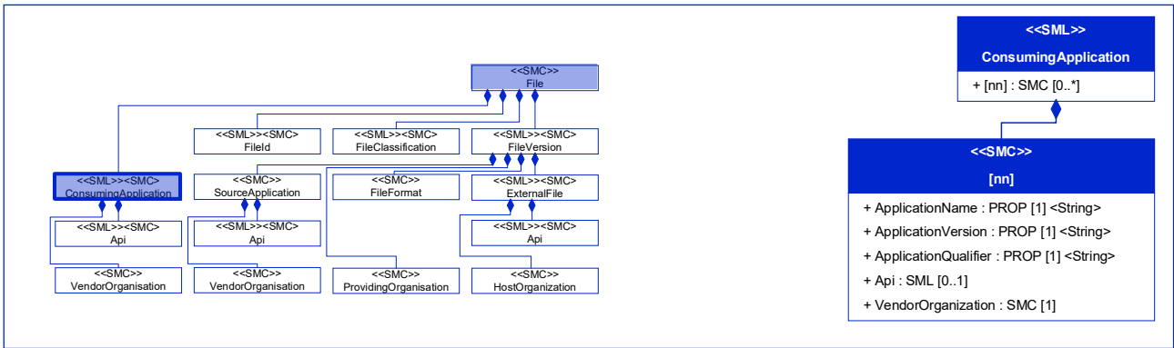
Figure 54: [Prop] ApplicationName
