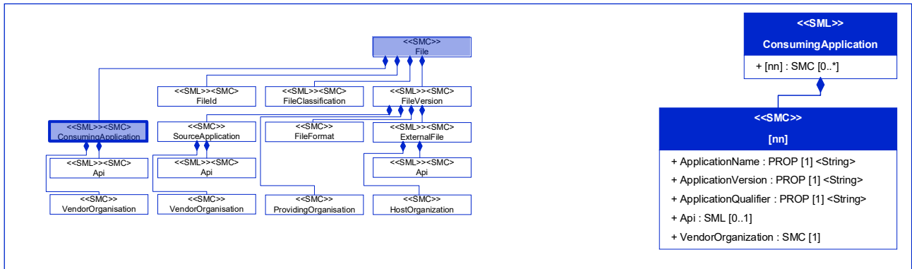
Figure 56: [Prop] ApplicationQualifier
