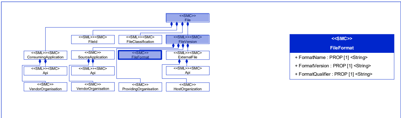
Figure 37: [Prop] FormatVersion
