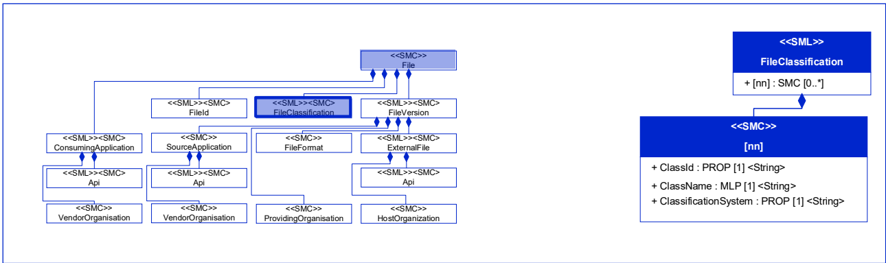
Figure 67: [Prop] ClassificationSystem
