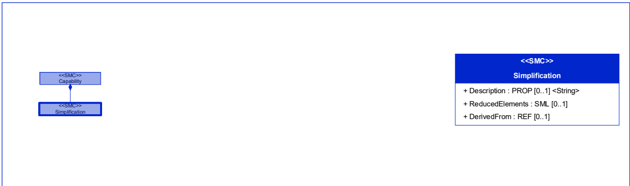
Figure 77: [Prop] Description
