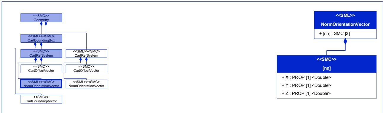
Figure 92: [Prop] X
