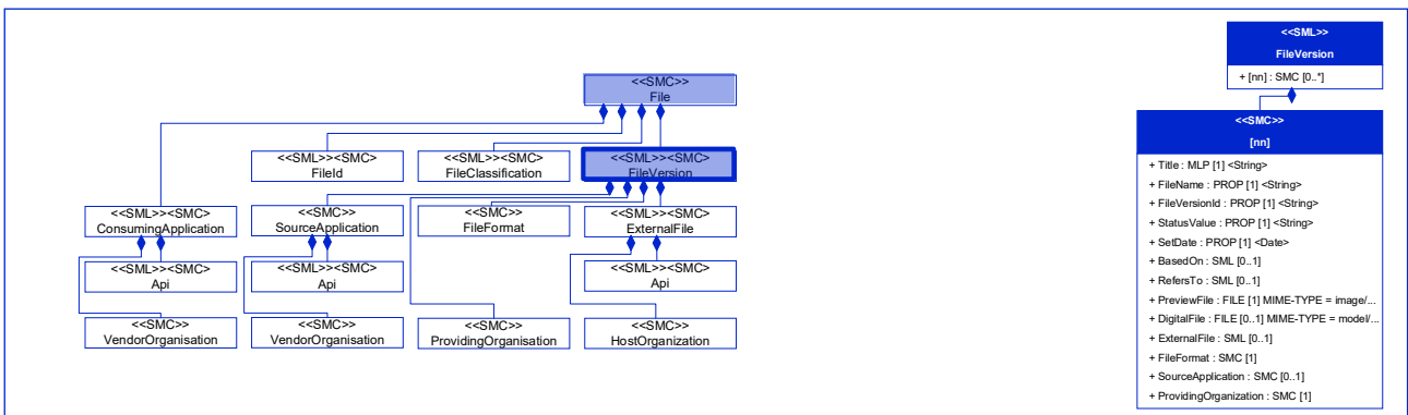
Figure 20: [Prop] SetDate
