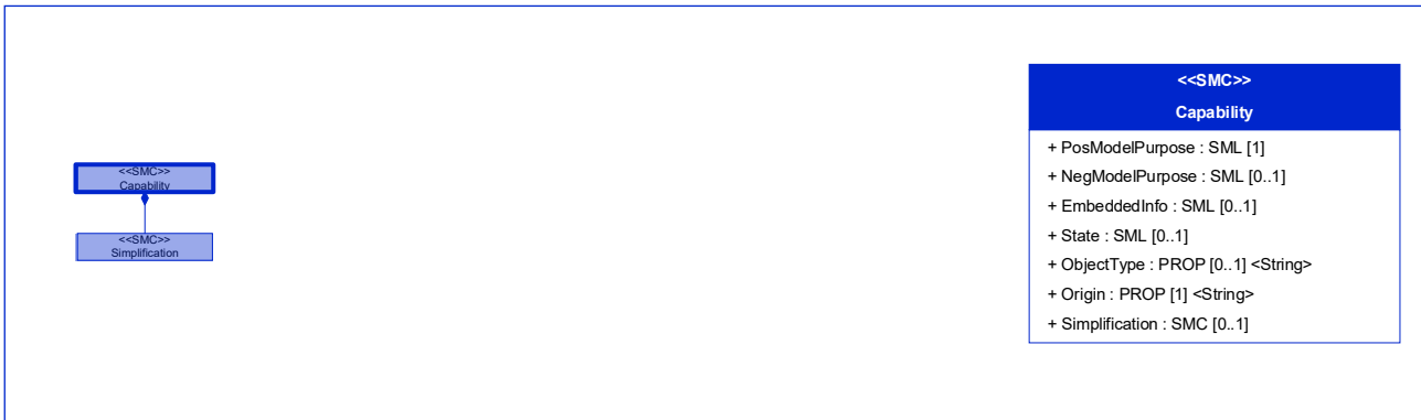
Figure 69: [SMC] Capability
