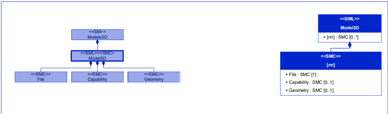
Figure 8: [SML][SMC] Model3D
