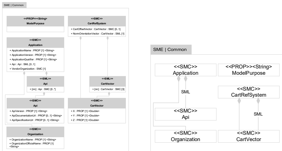
Figure 118: Common SubmodelElements [SME] within [SMT] Provision of 3D Models – Overview
