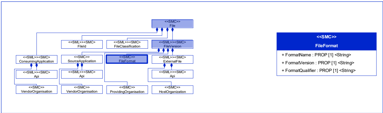
Figure 36: [Prop] FormatName
