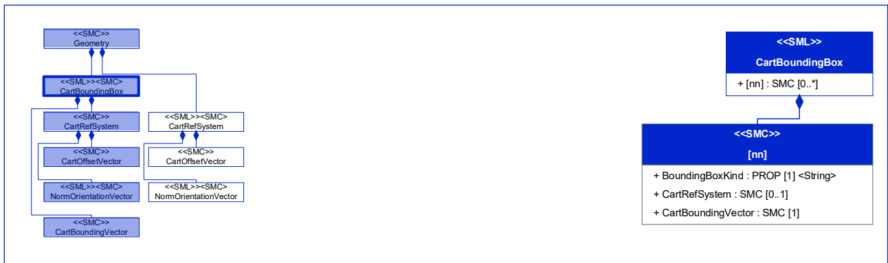
Figure 84: [SML][SMC] CartBoundingBox
