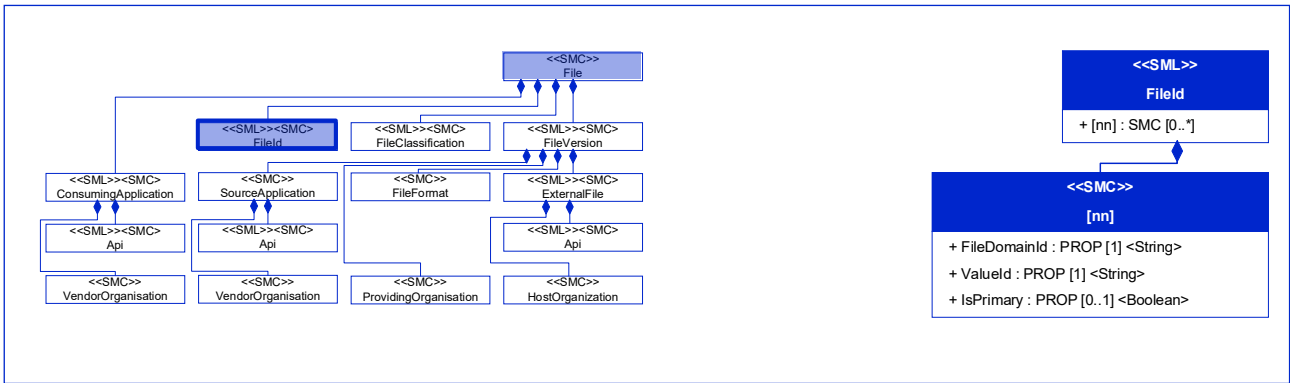
Figure 12: [Prop] FileDomainId
