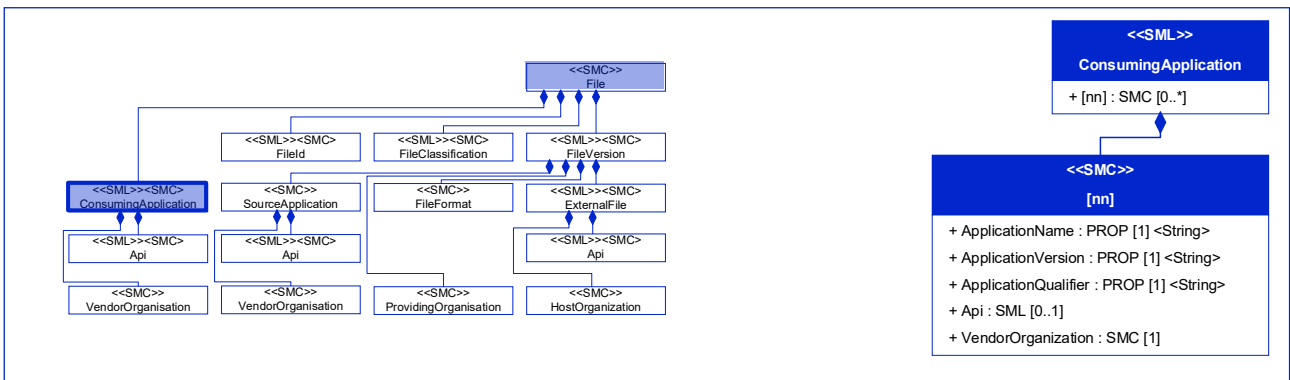
Figure 55: [Prop] ApplicationVersion
