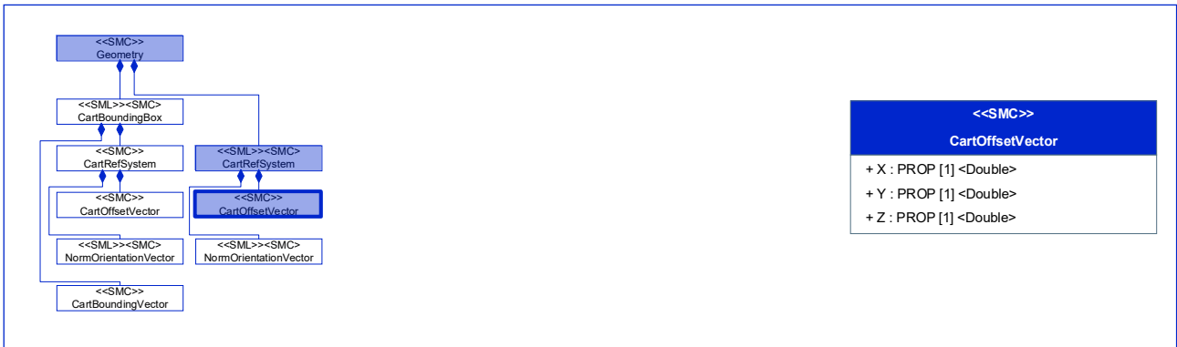
Figure 103: [Prop] Z
