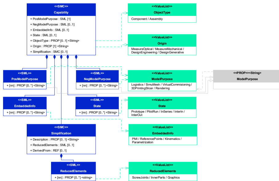
Figure 68: [SMC] Capability
