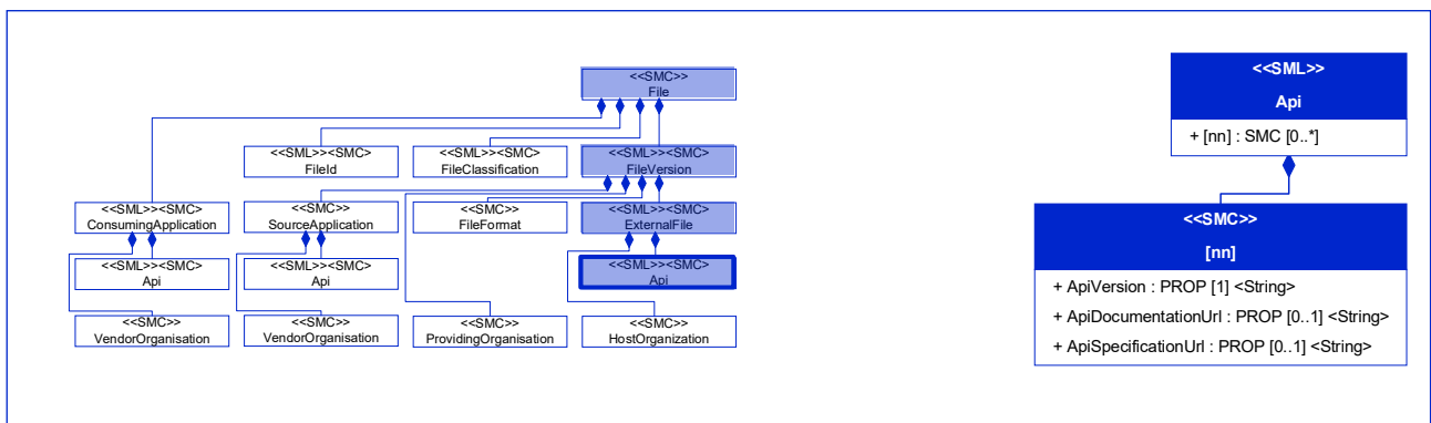
Figure 33: [Prop] ApiDocumentationUrl
