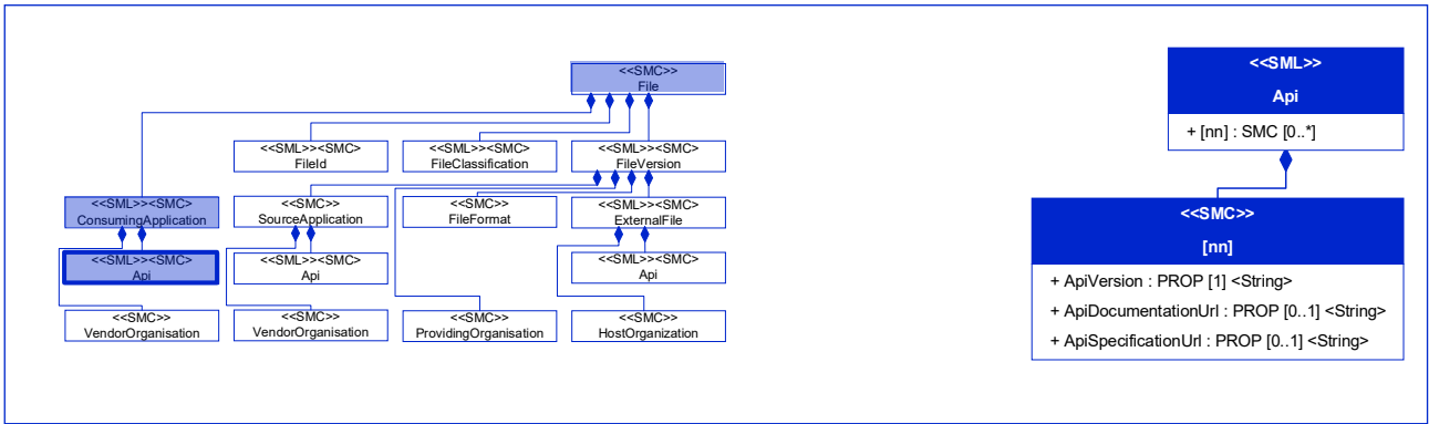
Figure 60: [Prop] ApiSpecificationUrl
