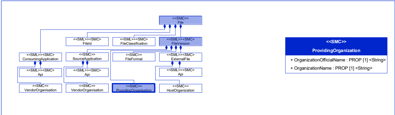
Figure 52: [Prop] OrganizationOfficialName
